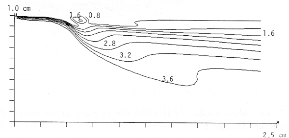
FIG. 9. Mach number contour on the xy plane at the center of the injection port for case 1.
