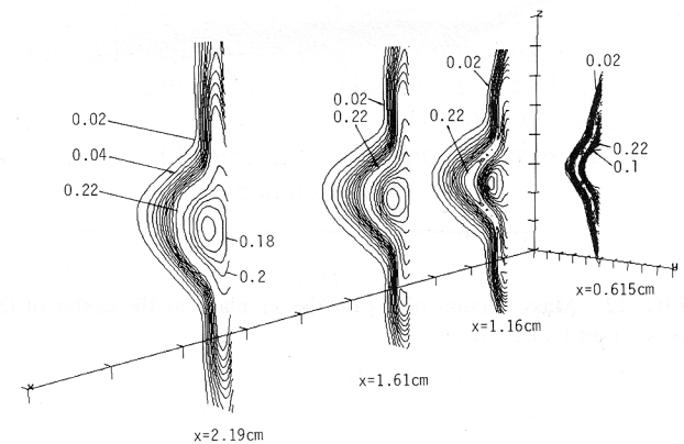
FIG. 8. Mass fraction of H_2O on yz planes at various x locations for case 1.
