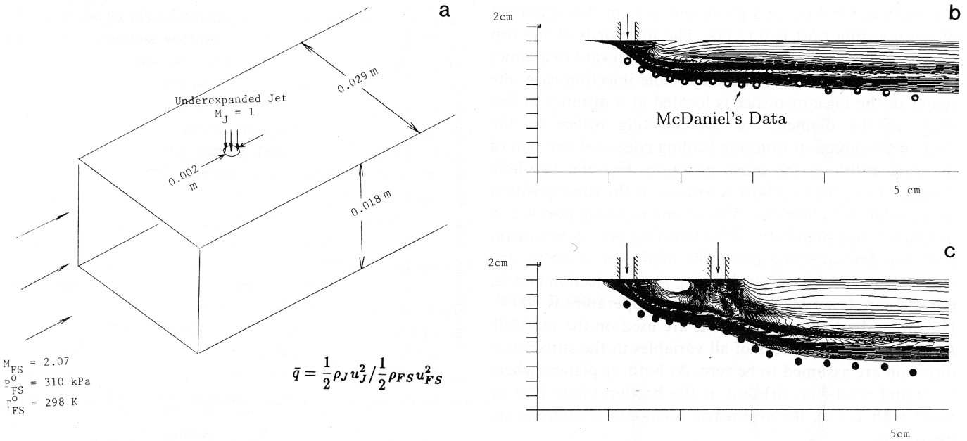
FIG. 2. McDaniel's Experiment: (a) geometry; (b) comparison of predicted and experimental jet penetration for single-port injection; (c) comparison of predicted and experimental jet penetration for dual-port injection.
