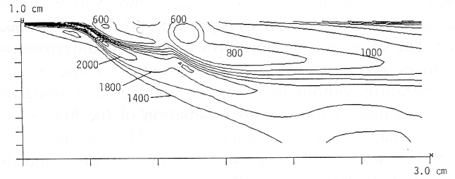
FIG. 15. Temperature contour on the xy plane at the center of the injection port for case 2.
